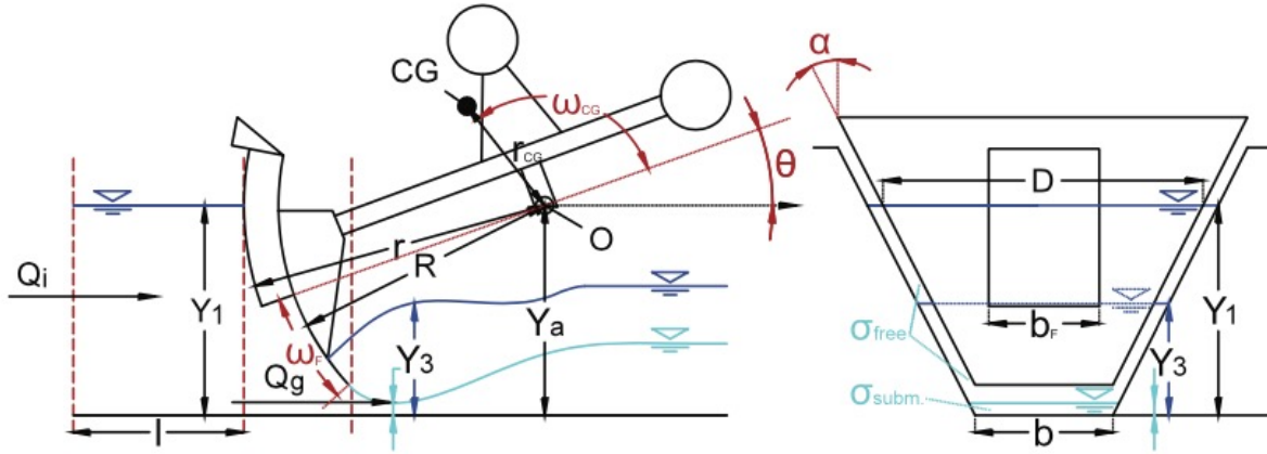
Fig. 2. (Color) Longitudinal and cross-section illustration of gate giving the geometric parameters
