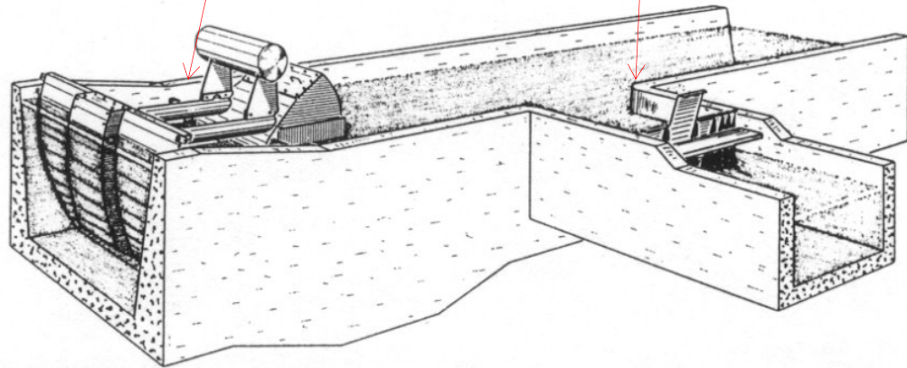
Valves with constant downstream level
